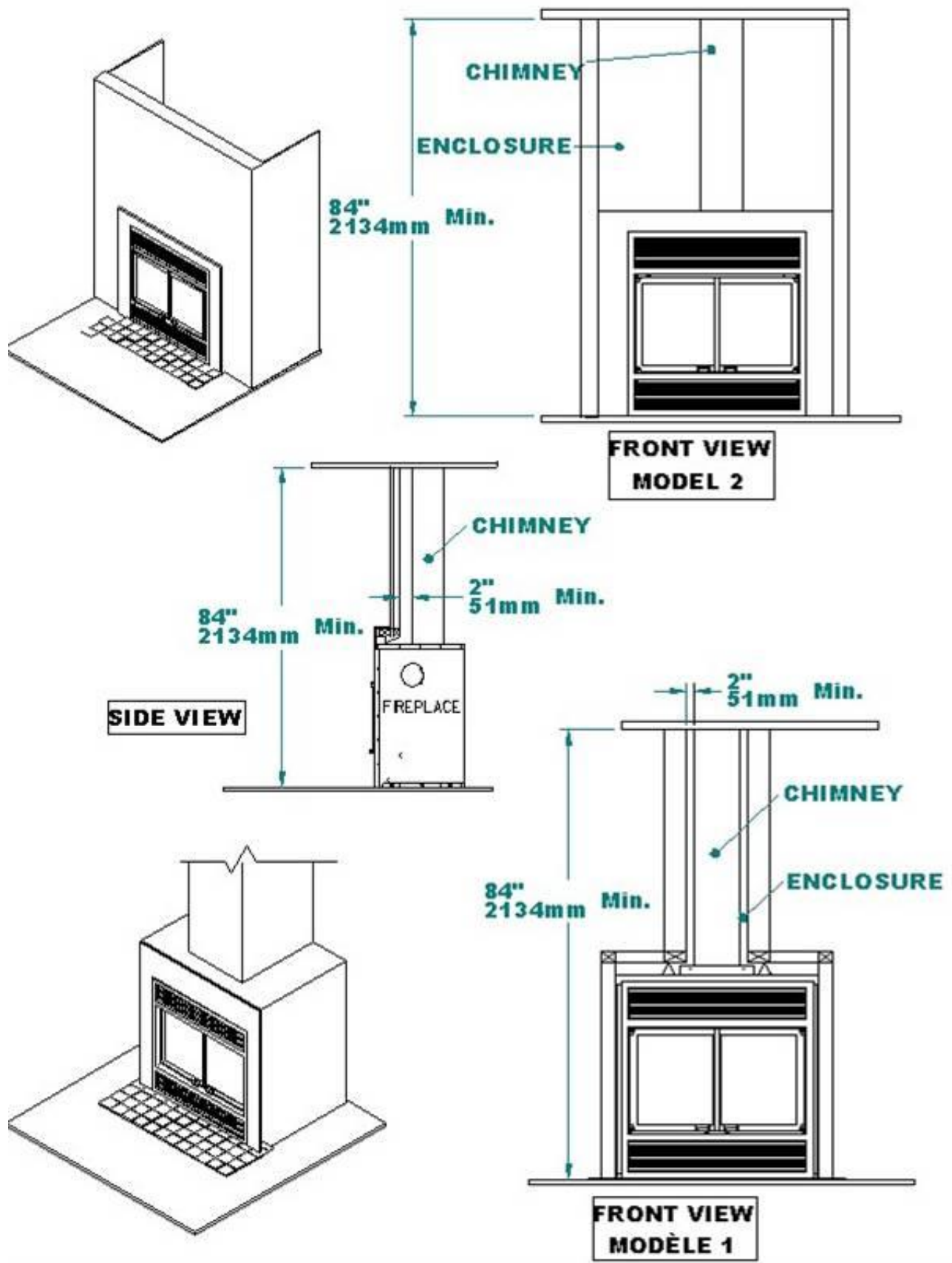
Figure #15: Chimney Enclosure
