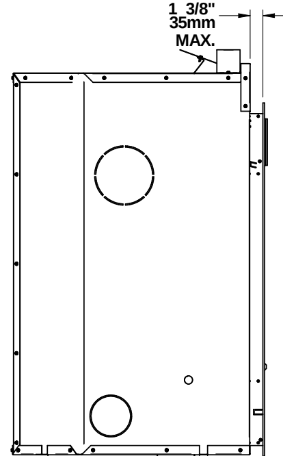
SECTION B-B
