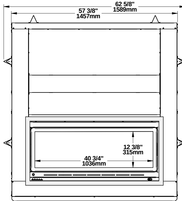
SECTION F-F
