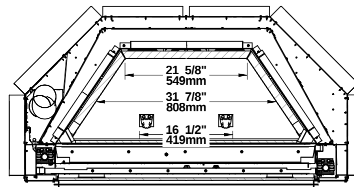
SECTION G-G
