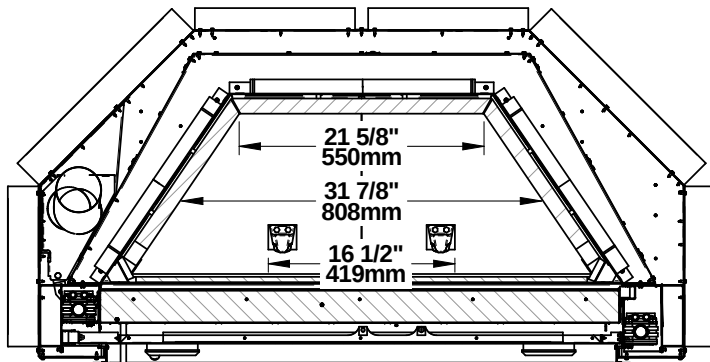
SECTION F-F
