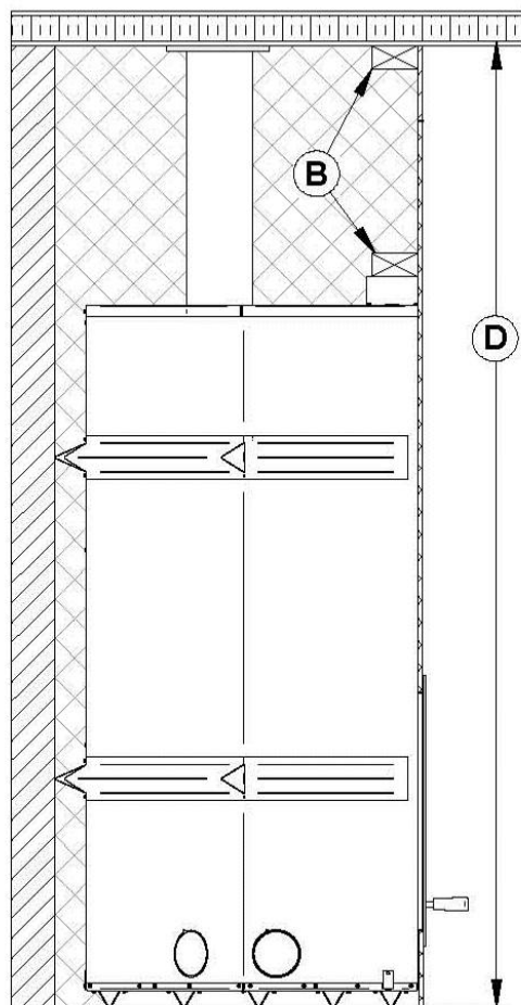
Figure 19 : Framing
