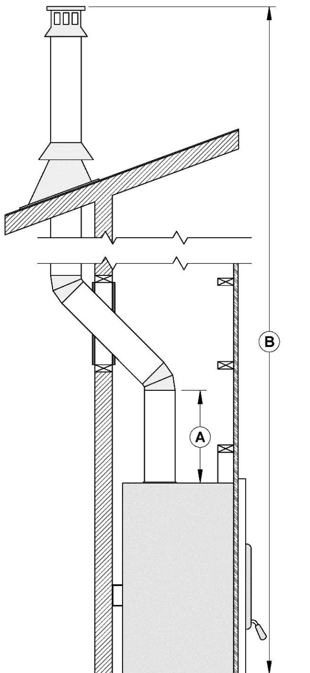
Figure 48 : Typical Installation
