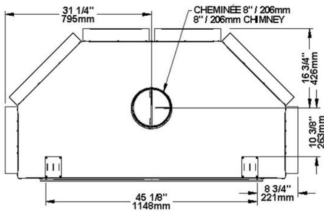
Figure 1 : Top View
