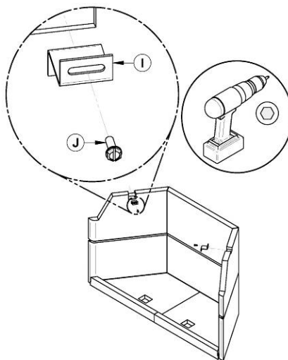
Figure 39 : Panels Retainers
