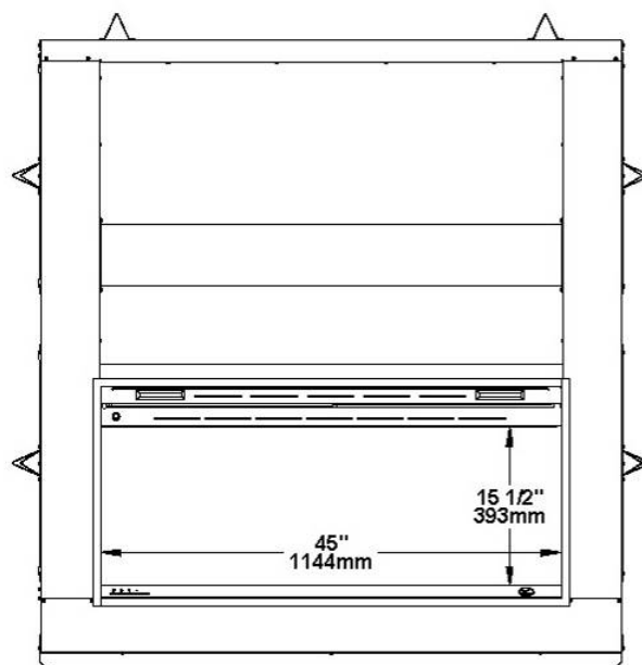
Figure 8 : Door Opening Straight masonry trim
