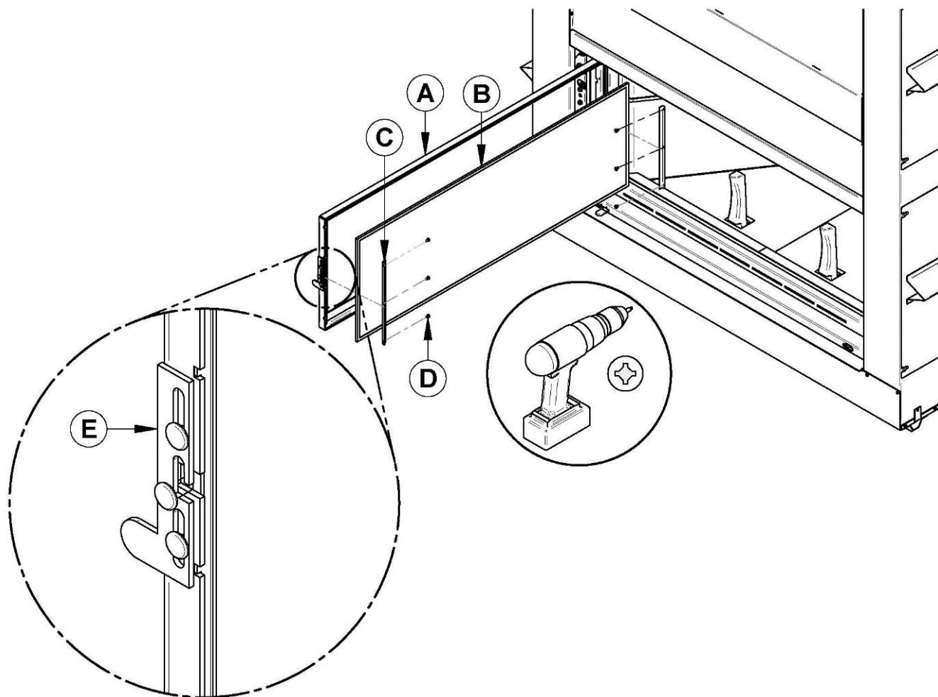
Figure 56 : Glass replacement
