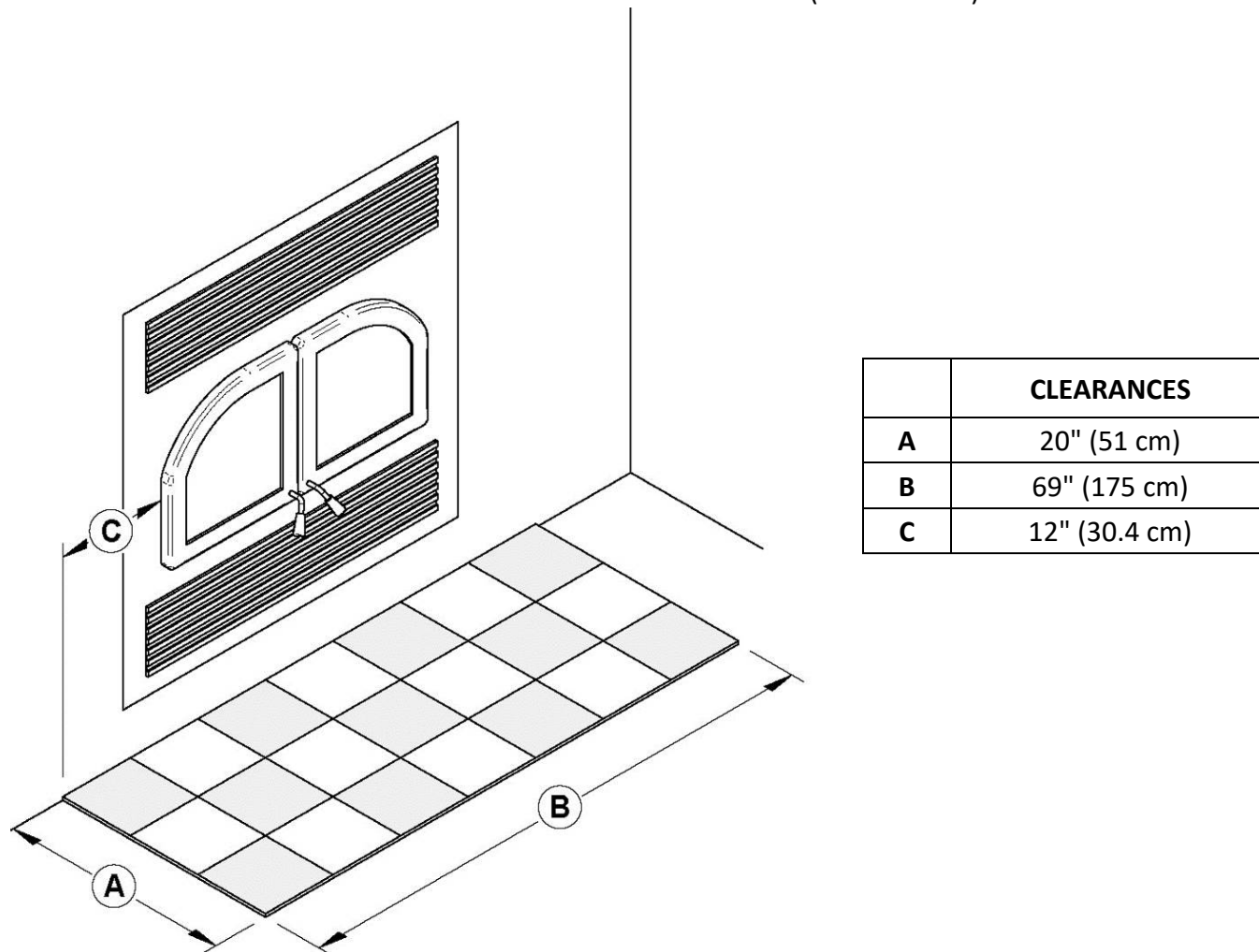
Figure 18 : Hearth Extension Dimension
