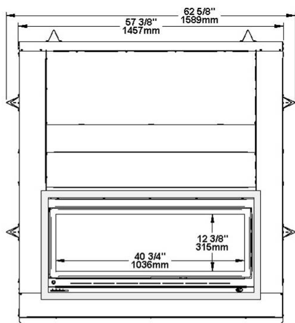
Figure 5 : Glass surface
