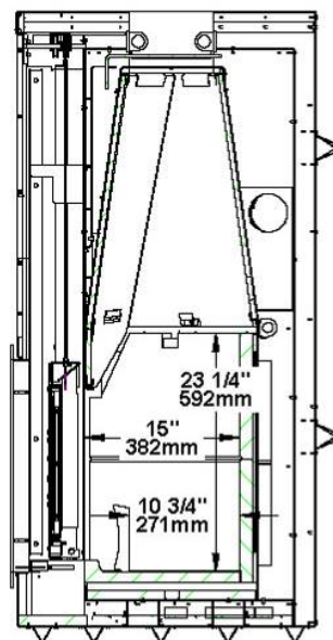
Figure 6 : Combustion chamber
