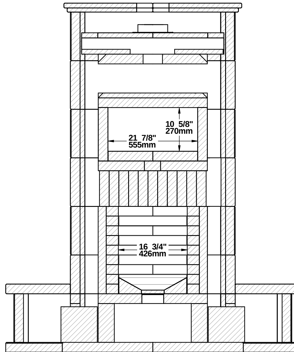
SECTION B-B
