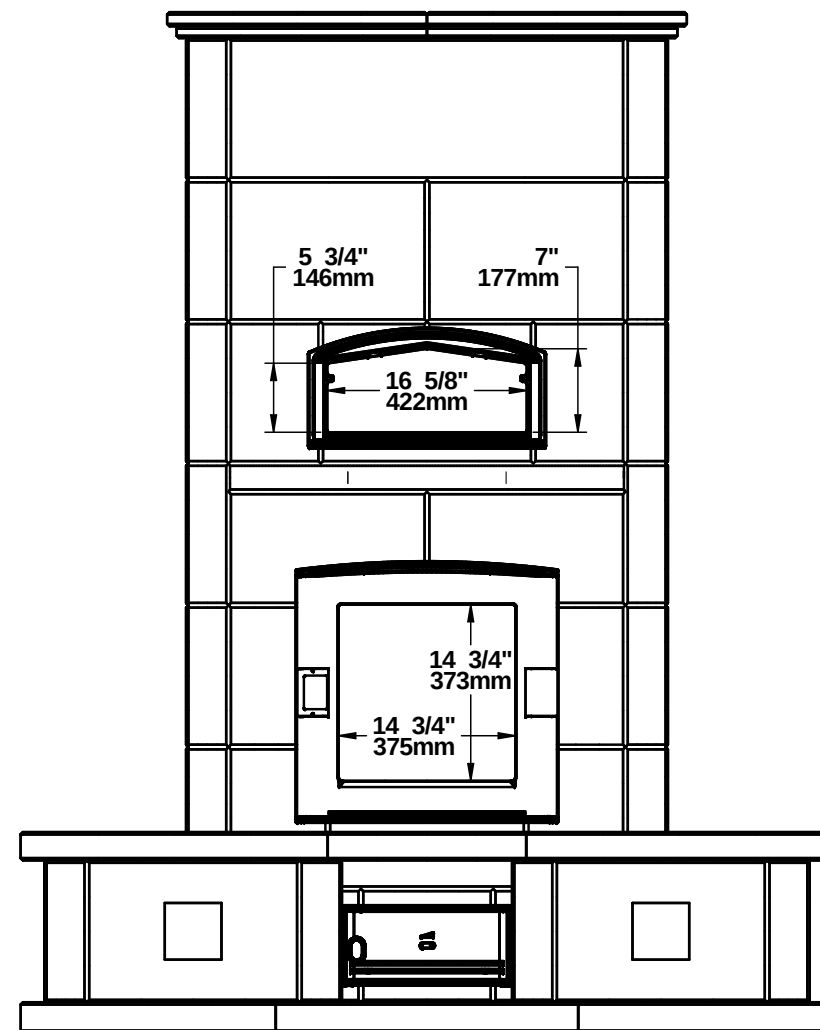
SECTION C-C
