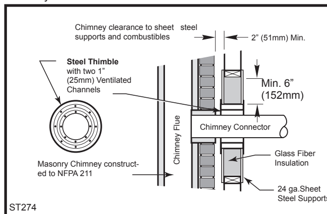
Fig. 11 Wall Pass-through using single wall chimney connector with a ventilated steel thimble.
