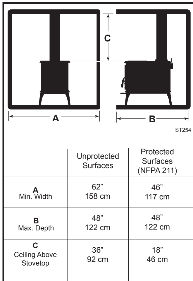
Fig. 21 Alcove Specifications.
