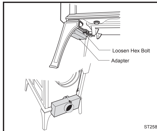
Fig. 24 Attach the adapter to the bottom plate.
