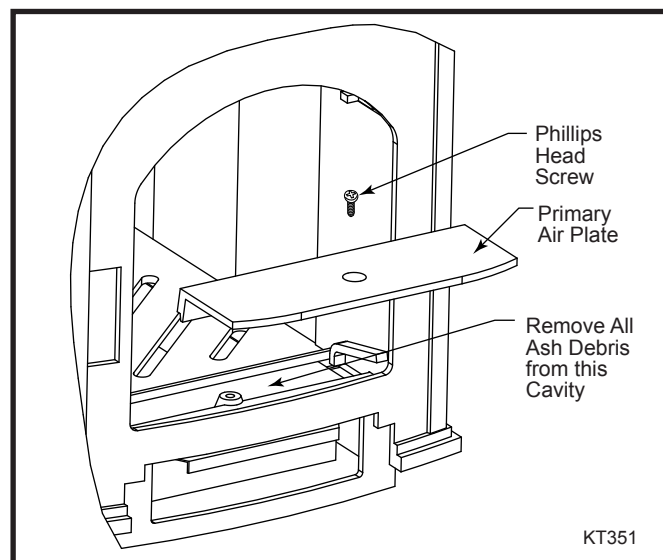
Fig. 34 Remove phillips head screw and primary air plate to clean ash from cavity.
