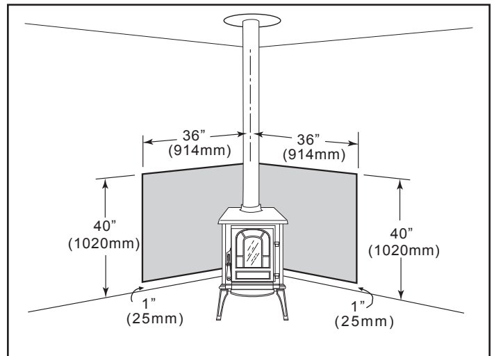
Figure 4.7 - Corner installation, vertical chimney connector, two wall shields.
