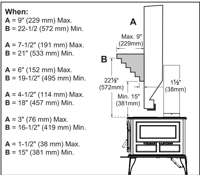
Figure 3.10 - Mantel and trim clearances.
