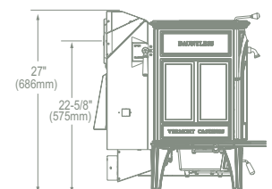
Side - Rear Vent
