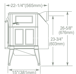
Side - Rear Vent
