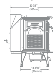
Side - Top Vent
