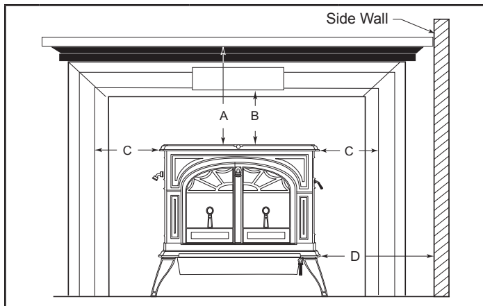
Fireplace and Mantel Trim Clearances
