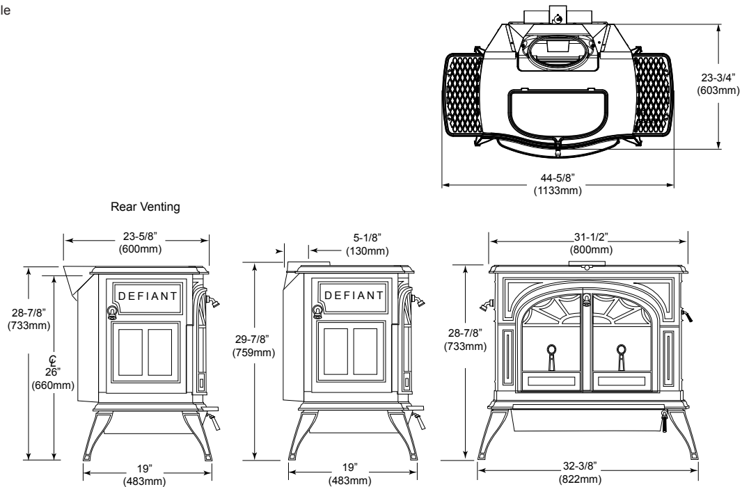
Figure 1 - Defiant® 1975 dimensions.
