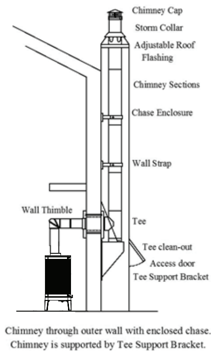
Figure 9 – Typical Chimney Configurations
