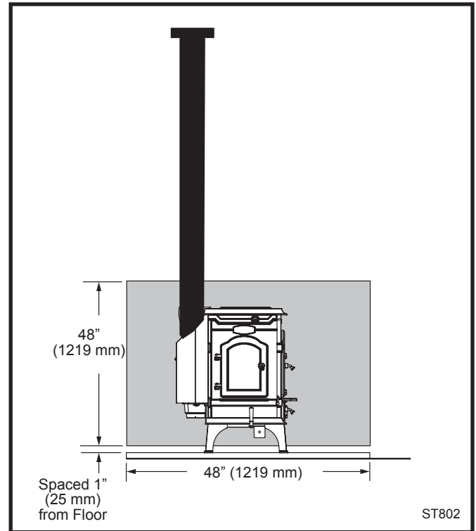
Fig. 17 Sidewall protection.
