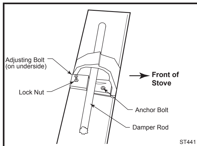
Fig. 33 Damper adjustment.
