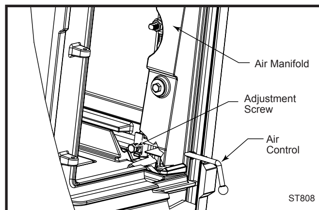
Fig. 34 Primary air control adjustment.
