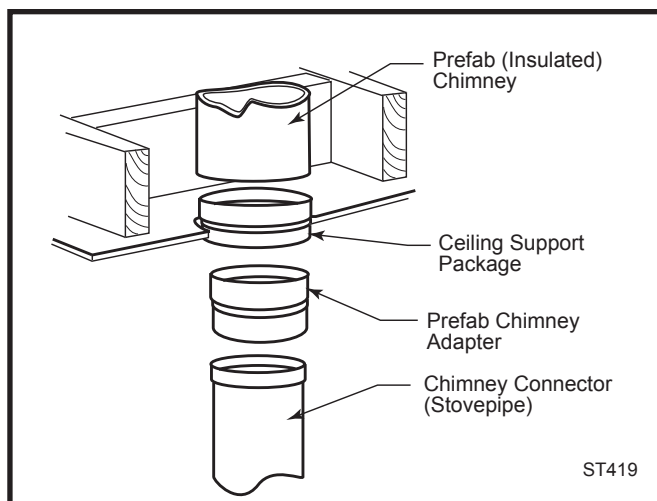
Fig. 6 Joining the chimney connector to a prefabricated chimney.
