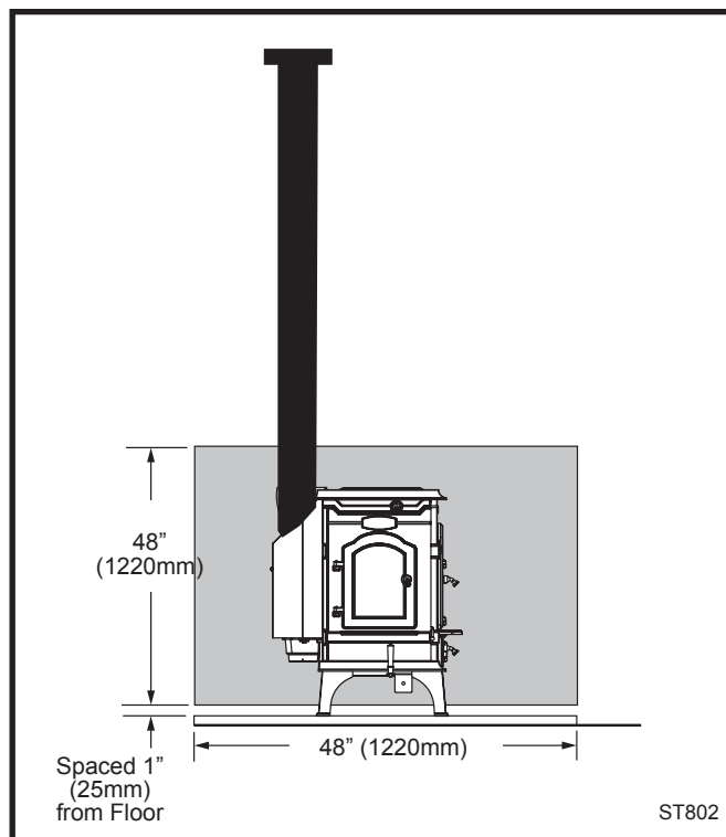
Fig. 22 Sidewall protection.
