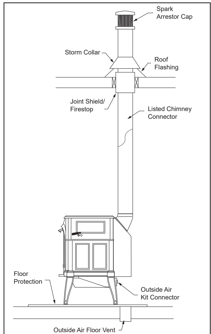
Figure 2.17 - Mobile home installation.
