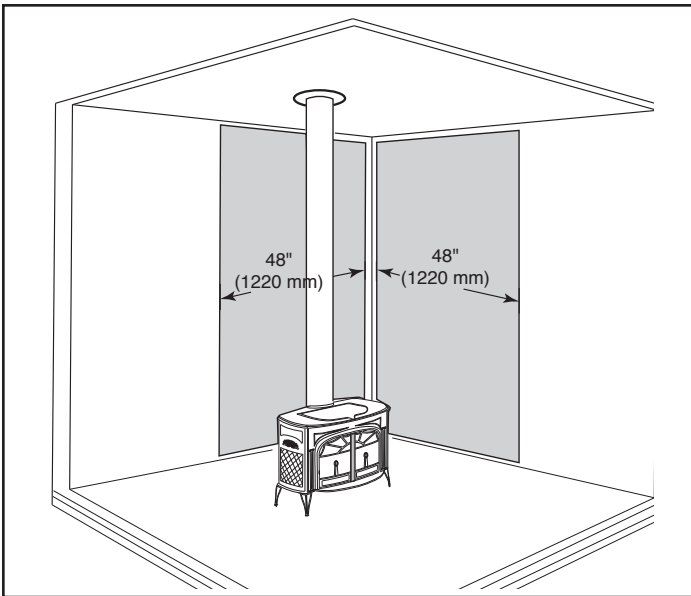
Figure 2.12 - Parallel installation, vertical chimney connector, two wall shields. Reduced clearances for both rear and side walls. Wall shields may meet at corner if desired. Shielding for connector is centered behind connector.
