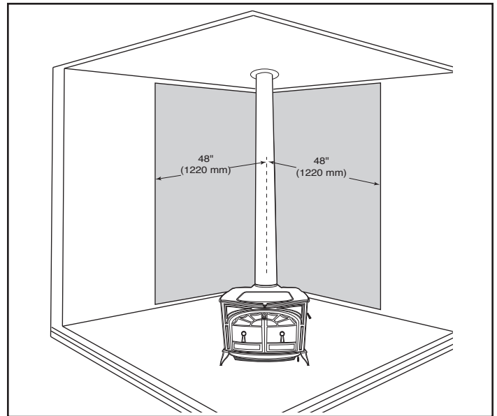
Figure 2.14 - Corner installation, vertical chimney connector, two wall shields. Reduced side clearances. Wall shield MUST meet at corner.
