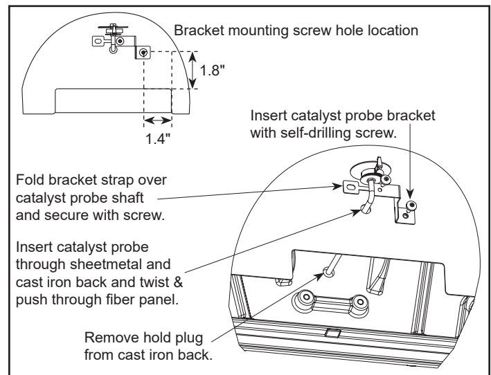
Figure 3.7 - Install the Catalyst Temperature Probe
