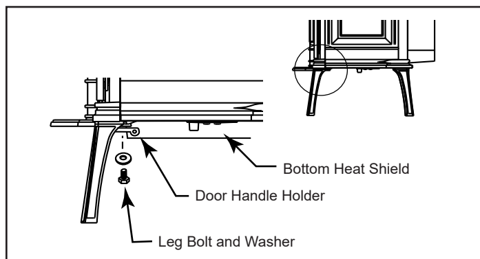
Figure 3.4 - Handle holder and heat shield positions.
