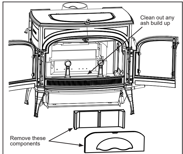
Figure 6.6 - Inspect and clean out ash accumulation behind the combustion system.
