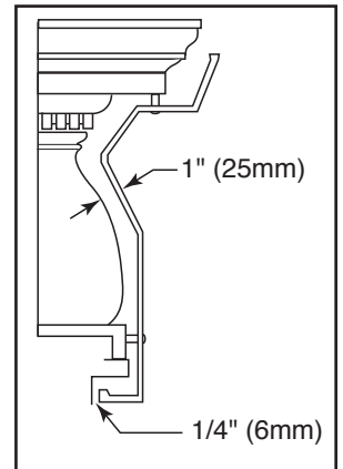
Figure 2.15 - A custom-formed mantel shield.
