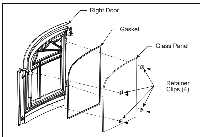
Figure 6.1 - Exploded view of the glass assembly for the right door.
