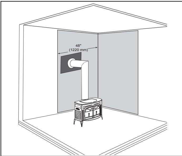
Figure 2.13 - Parallel installation with rear wall pass-through, two wall shields. Reduced clearances to both rear and side walls. Wall shields may meet at corner if desired. Wall pass-through must comply with codes.
