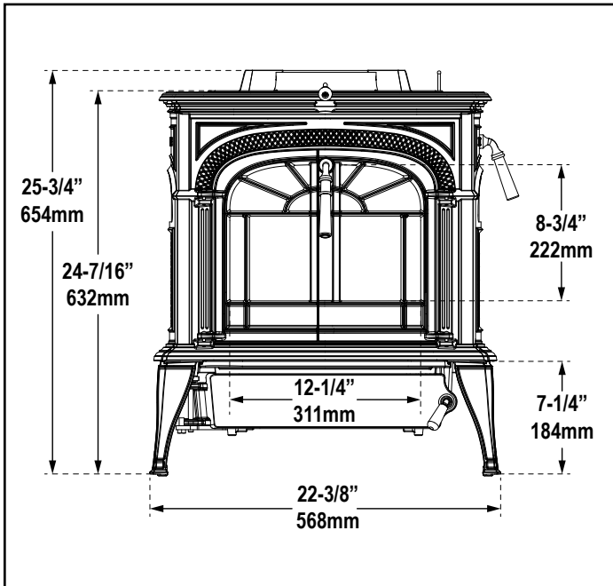
Figure 3.1 - Front View
