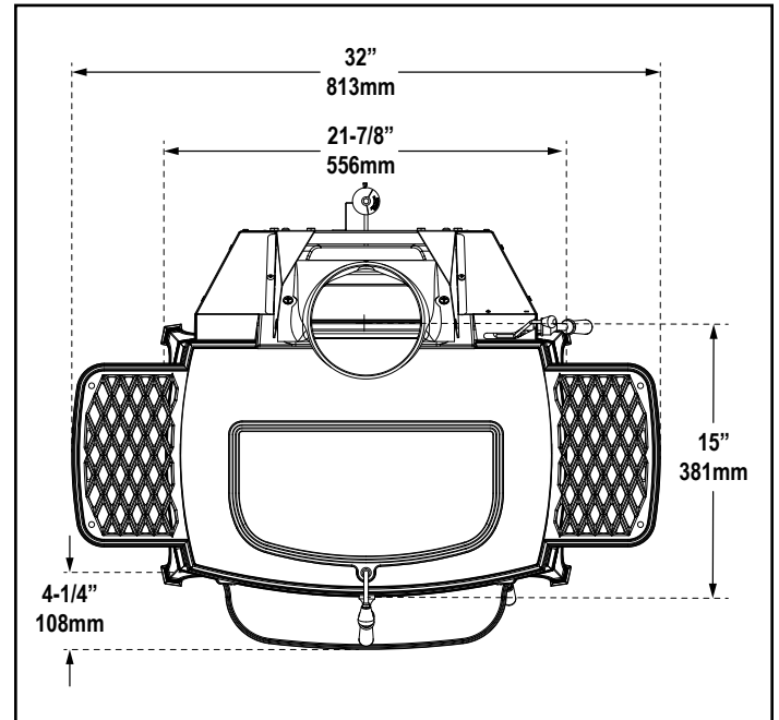
Figure 3.2 - Top View
