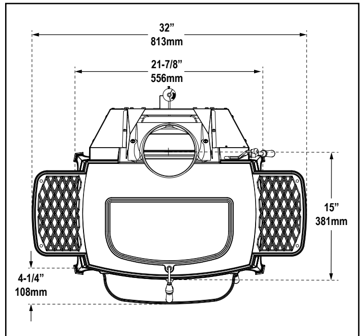
Figure 3.2 - Top View
