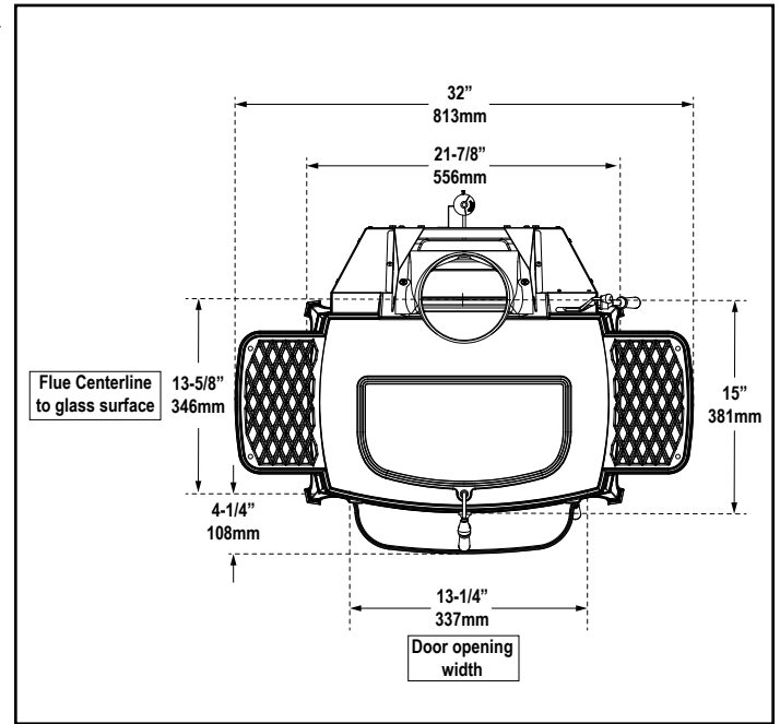
Figure 3.3 - Top View
