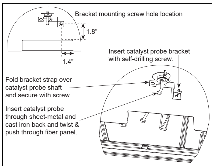
Figure 5.9 - Install the Catalyst Temperature Probe
