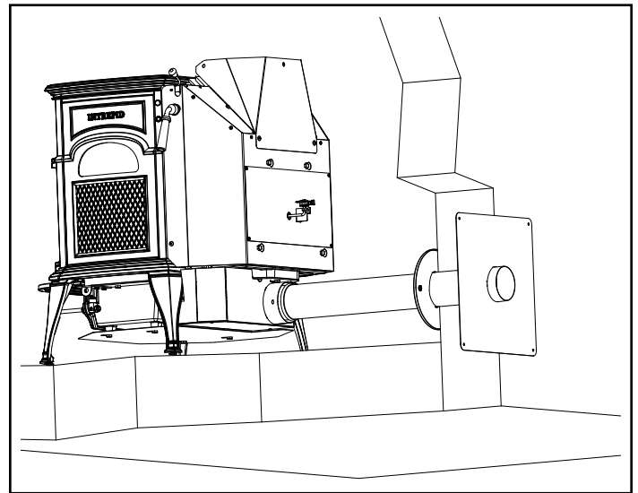
Figure 5.13 - Rear Installation
