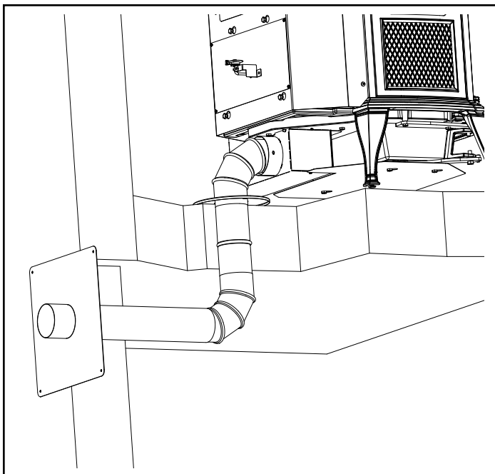
Figure 5.14 - Floor Installation
