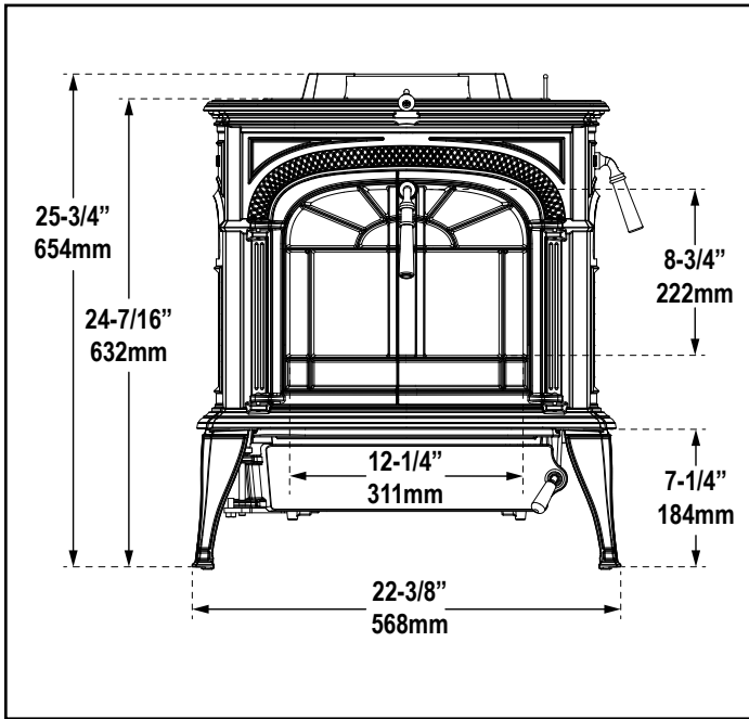
Figure 3.1 - Front View
