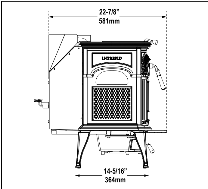
Figure 3.2 - Side View
