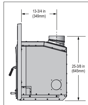
Figure 9.5 - Side View with Cast Surround (MED-CB or MED-BN) and Optional 15 Degree Adapter (DV-6DLR-E15ADSS)
