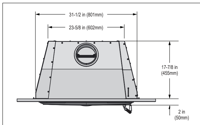
Figure 8.1 - Top View with Small Surround (SPVC-4331)
