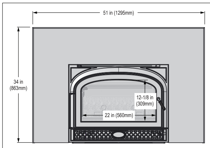
Figure 8.5 - Front View with large Surround (SPVC-5134)
