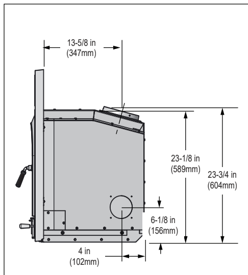
Figure 9.3 - Side View with Cast Surround (MED-CB or MED-BN)
