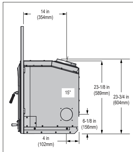
Figure 8.6 - Side View with Large Surround (SPVC-5134)
