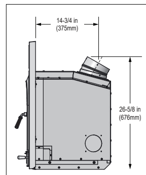
Figure 9.7 - Side View with Cast Surround (MED-CB or MED-BN) and Optional 15 Degree Adapter set at 30° (DV-6DLR-E15ADSS)
