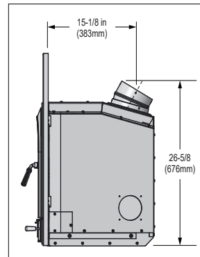
Figure 9.6 - Side View with Small or Large Surround (SPVC-4331 or SPVC-5134) and Optional 15 Degree Adapter set at 30° (DV-6DLR-E15ADSS)
