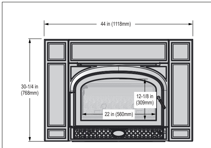
Figure 9.2 - Front View with Cast Surround (MED-CB or MED-BN)
