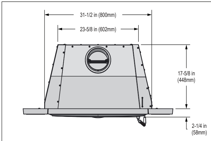
Figure 9.1 - Top View with Cast Surround (MED-CB or MED-BN)
