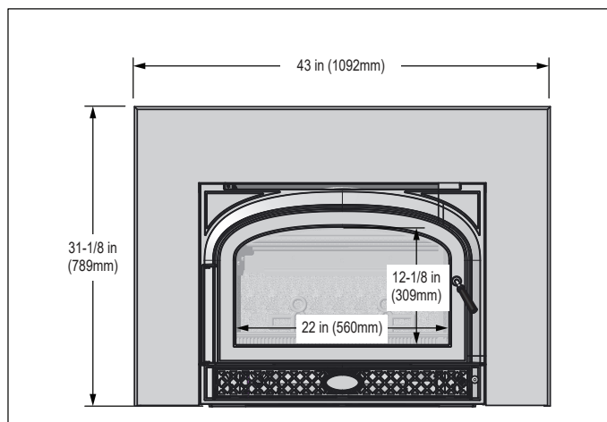
Figure 8.2 - Front View with Small Surround (SPVC-4331)
