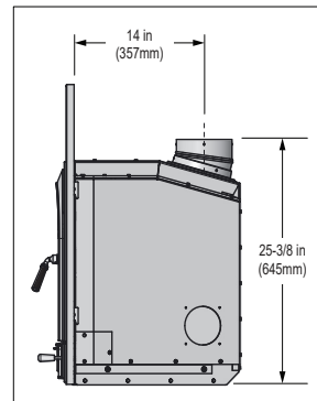
Figure 9.4 - Side View with Small or Large Surround (SPVC-4331 or SPVC-5134) and Optional 15 Degree Adapter (DV-6DLR-E15ADSS)
