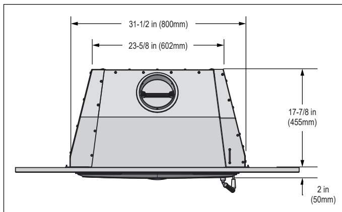
Figure 8.4 - Top View with Large Surround (SPVC-5134)
