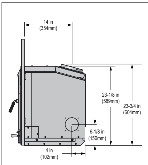
Figure 8.3 - Side View with Small Flat Surround (SPVC-4331)
