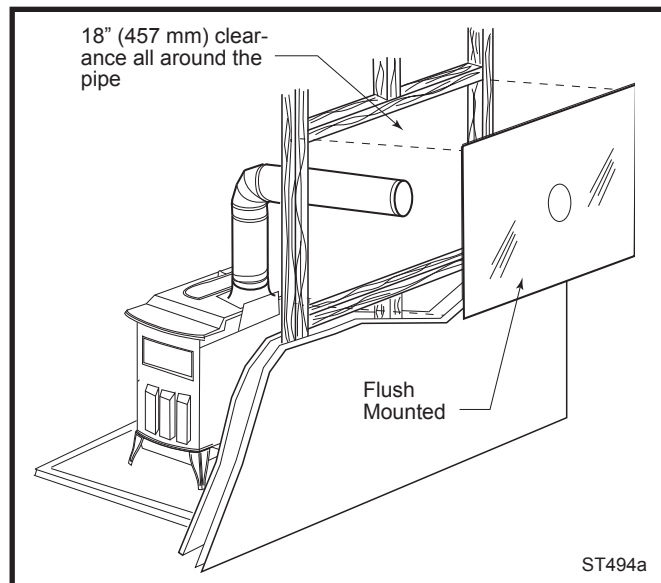
Fig. 10 An approved wall pass-through for Canada.
