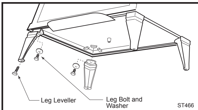
Fig. 26a Attach stove legs and leg levellers.
