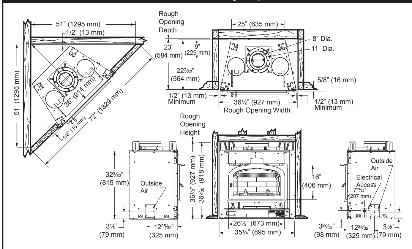
Fig. 1 Stratton specifications and framing.
