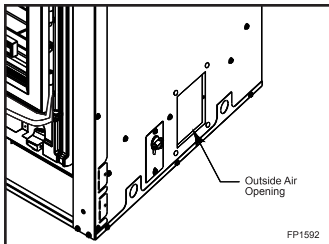
Fig. 16 Attach the inlet collar.
