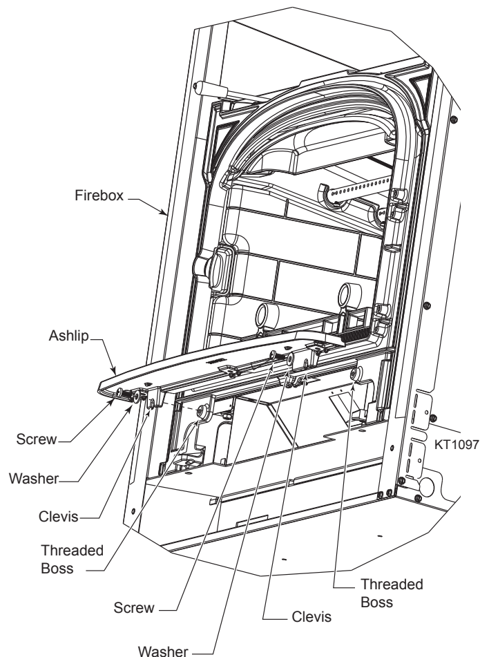
Fig. 36 Install ashlip.
