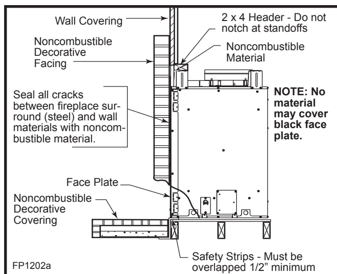
Fig. 33 Sealing gaps.
