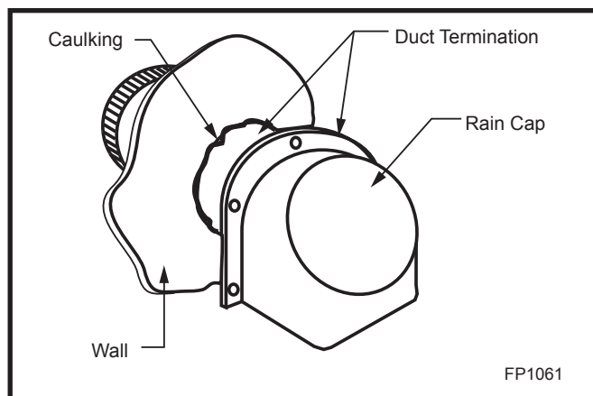
Fig. 17 Caulk and secure the duct termination/rain cap in place.
