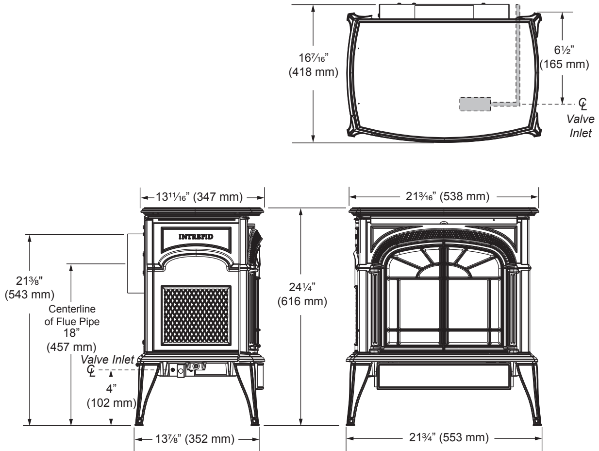
Fig. 1 Intrepid dimensions.
