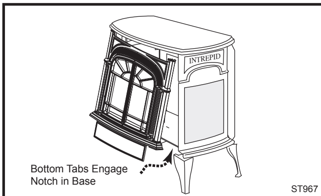
Fig. 57 Install stove front.
