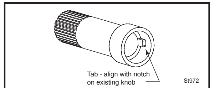
Fig. 66 Extension knob.
