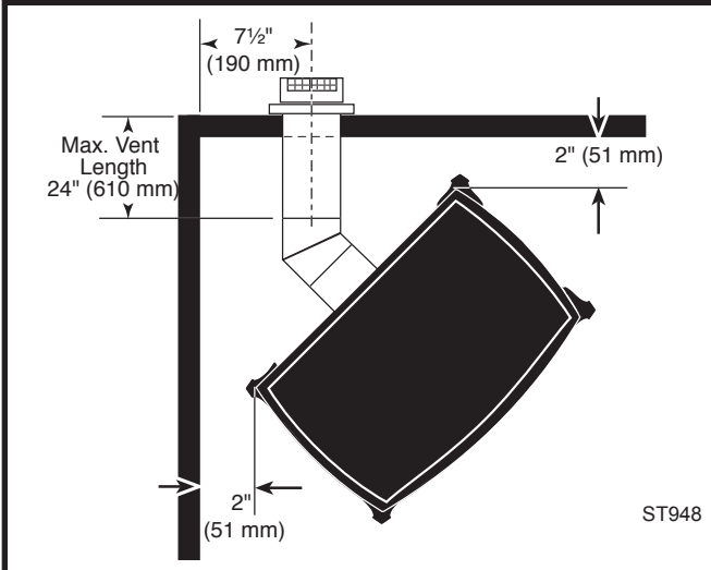
Fig. 4 Corner installation, minimum corner clearance and flue centerline.
