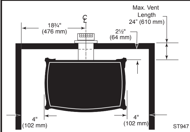
Fig. 3 Parallel Installation, minimum back and side clearance.
