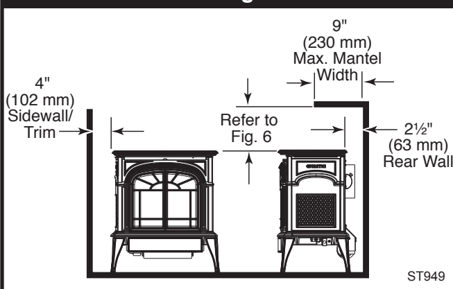
Fig. 5 Alcove and ceiling clearances.
