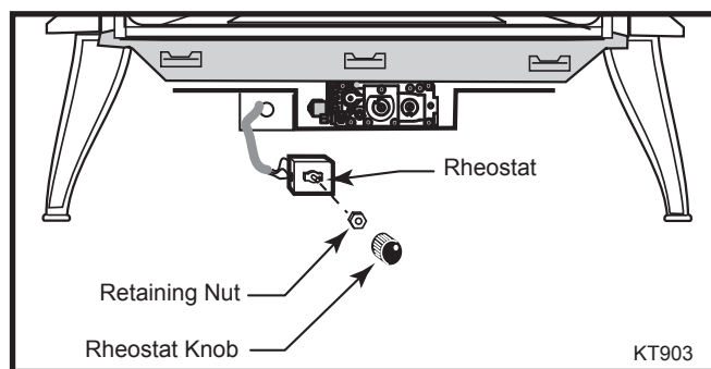
Fig. 17 Attach rheostat to bracket.
