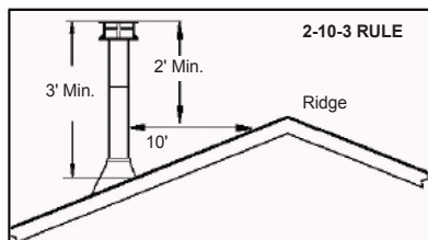
Figure 8 Chimney height requirements
