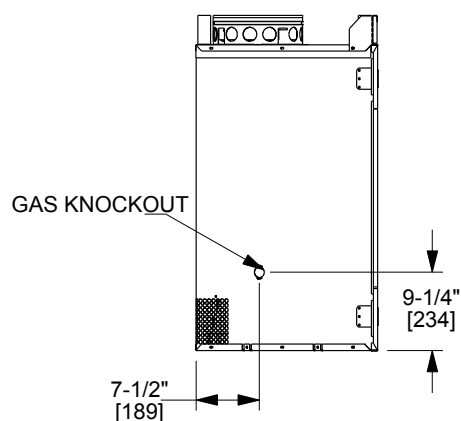
Left View
