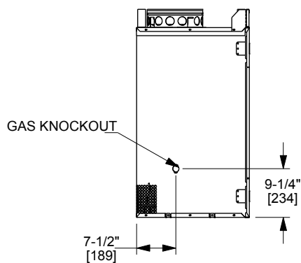
Left View
