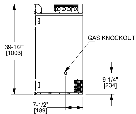
Right View
