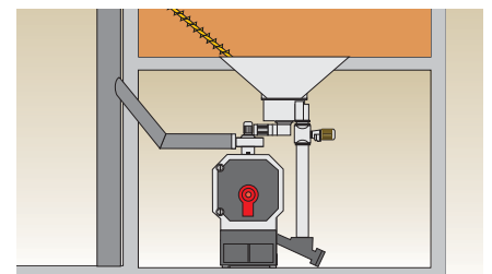
Silo funnel extraction
