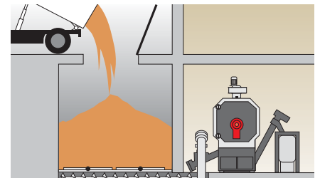
Bunker with walking floor
