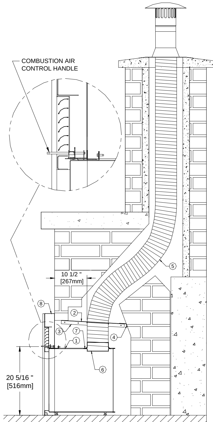
FIGURE 3 Installation
