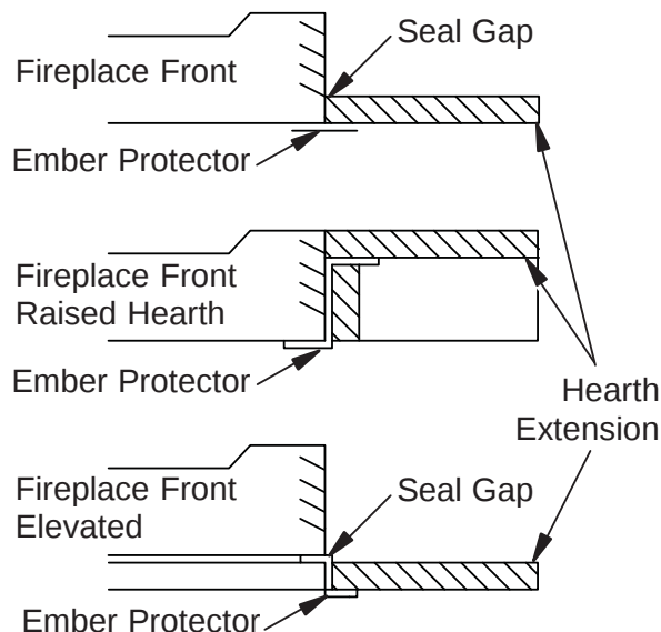
Figure 3 - Hearth Extension
