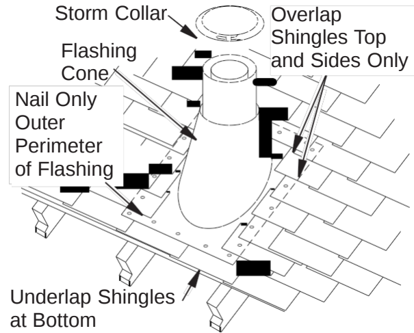
Figure 13 - Flashing Installation
