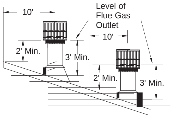
Figure 17 - 10 Foot Rule
