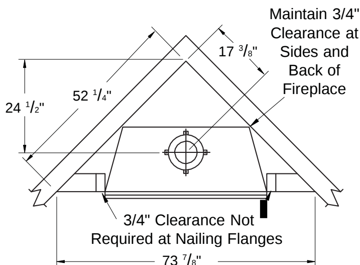
Figure 2 - Corner Installation
