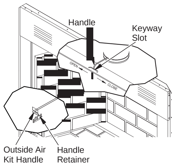
Figure 22 - Damper and Air Kit Handle
