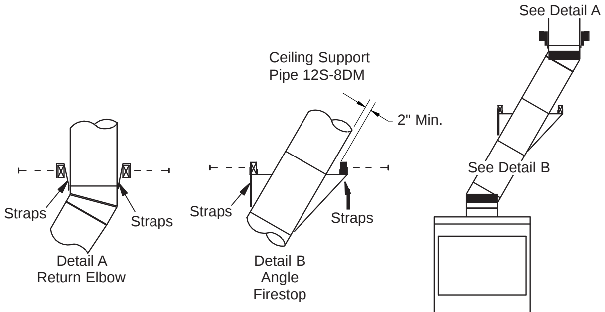
Figure 7 - Typical Offset Terminations
