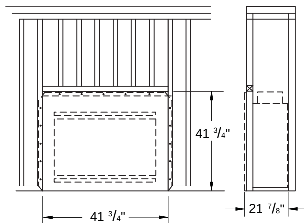
Figure 1 - Framing Dimensions
