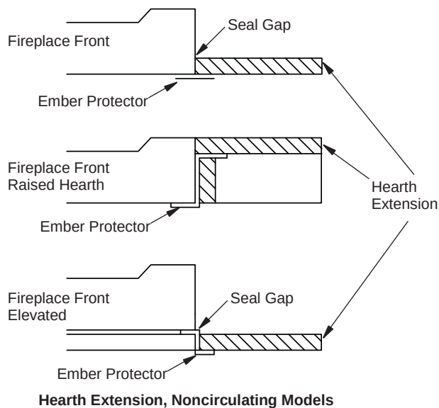
Figure 3 - Hearth Extension
