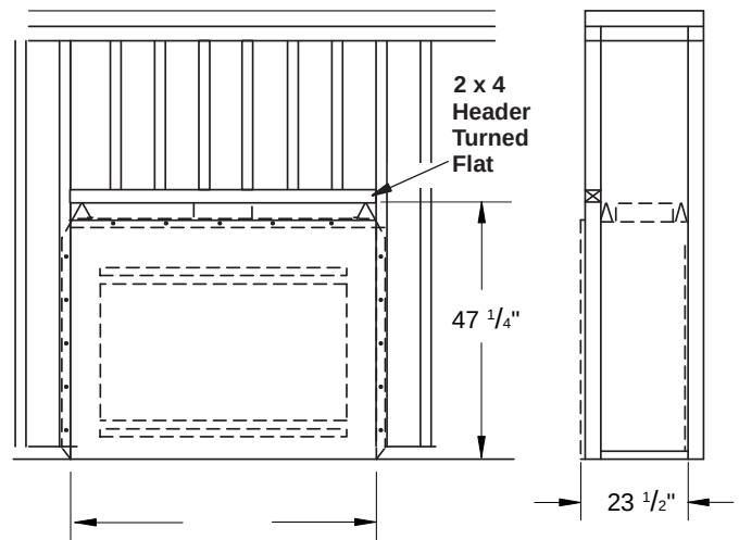
Figure 1 - Framing Dimensions
