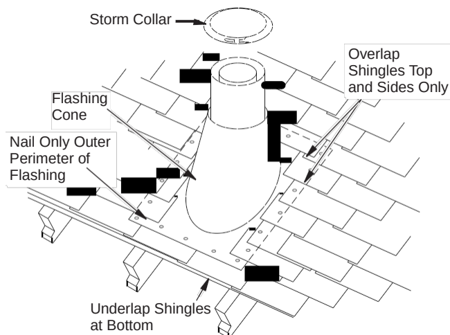
Figure 13 - Flashing Installation
