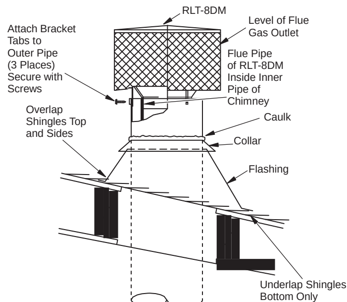
Figure 15 - Termination
