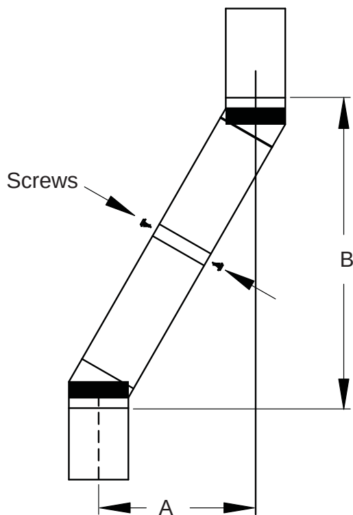
Figure 7 - Elbow Offset
