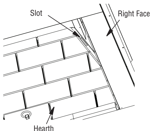
Figure 22 - Slots for Firebrick Walls
