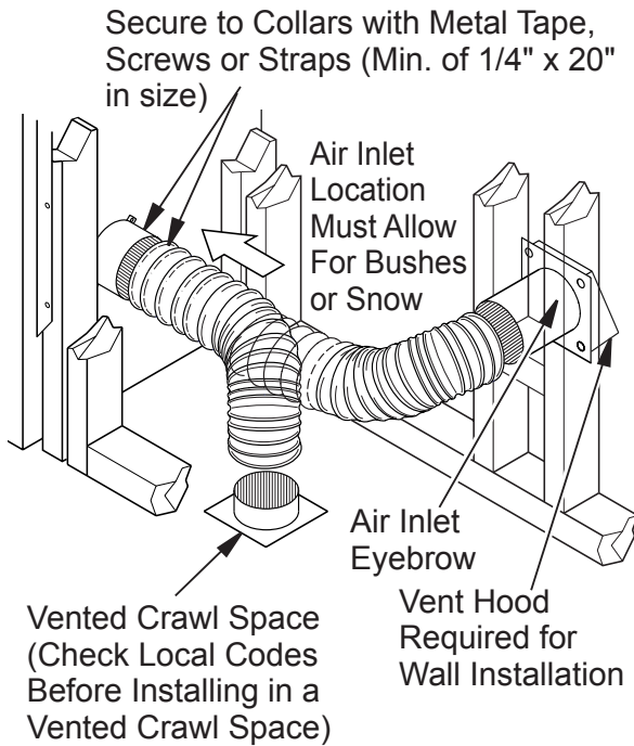
Figure 8 - Outside Air Kit
