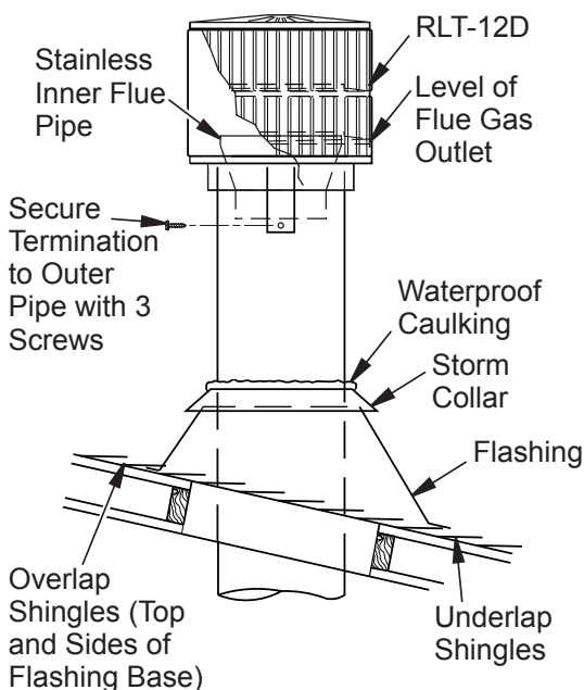
Figure 18 - Termination
