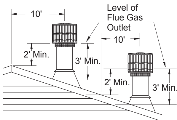
Figure 20 - 10 Foot Rule
