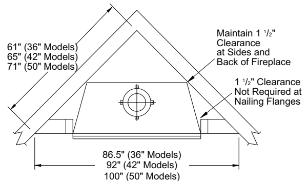
Figure 5 - Corner Installation
