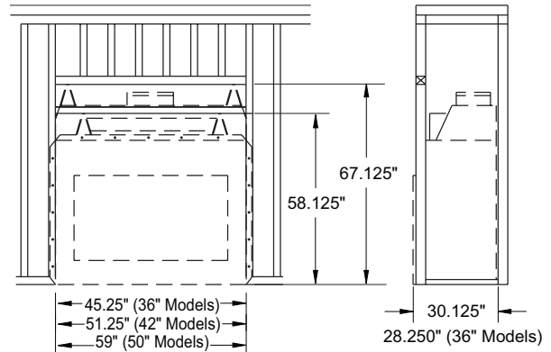
Figure 4 - Framing Dimensions
