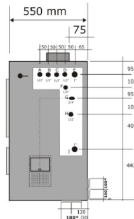
Hydraulic connections:
