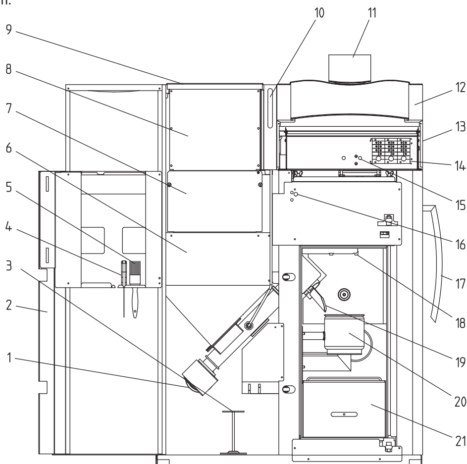
Fig. 4 BioWIN Klassik without combustion chamber door and with open cladding door
