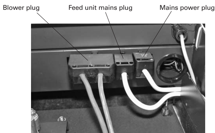
Fig. 145 Plug – rear of control panel
