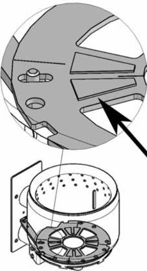
Fig. 124 BioWIN 210/260, Grate plate with embossing pointing upwards
