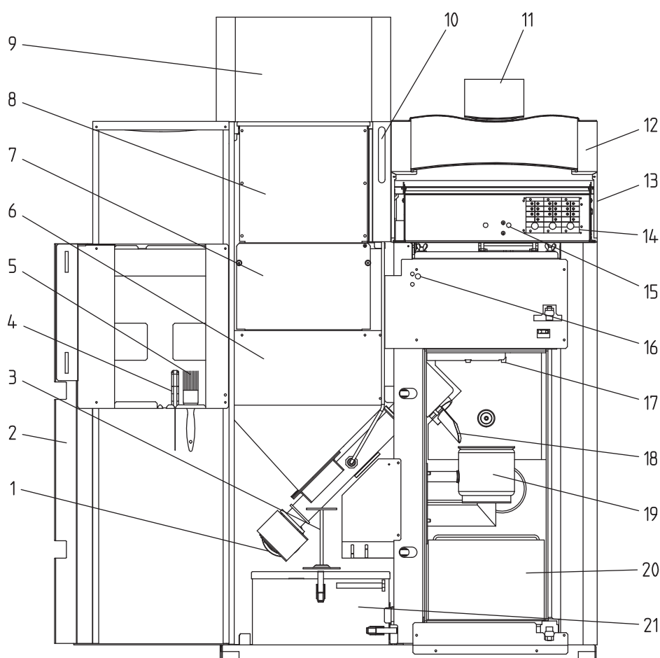
Fig. 6 BioWIN Exklusiv without combustion chamber door and with open cladding door
