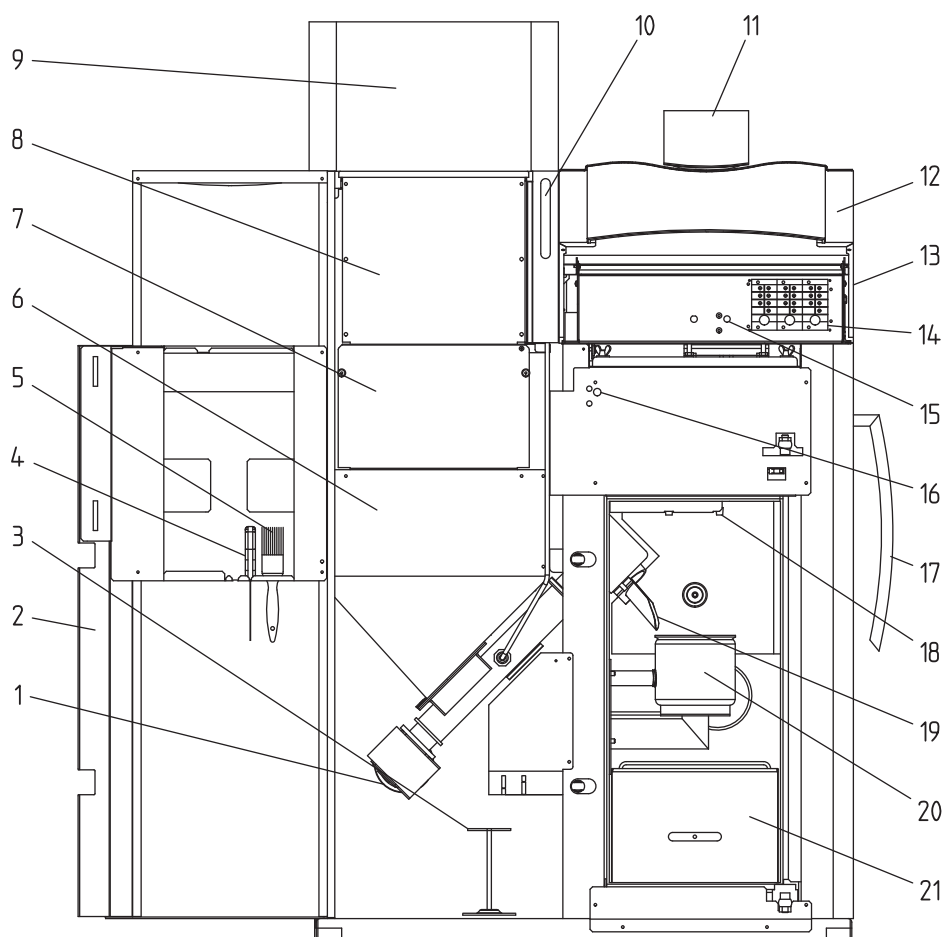
Fig. 5 BioWIN Premium without combustion chamber door and with open cladding door
