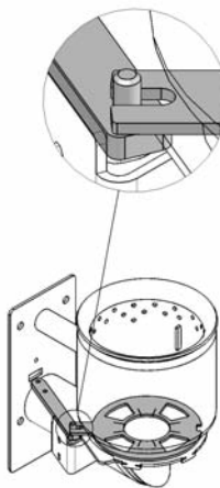
Fig. 123 BioWIN 100/150
