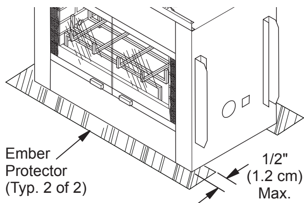
Figure 7 - Ember Protectors
