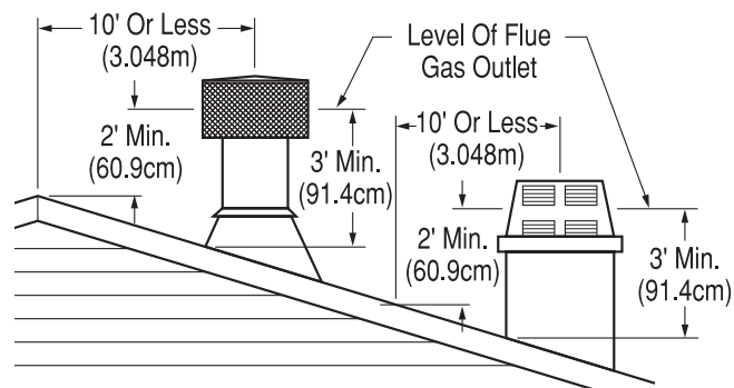
Figure 21- 10 Foot Rule
