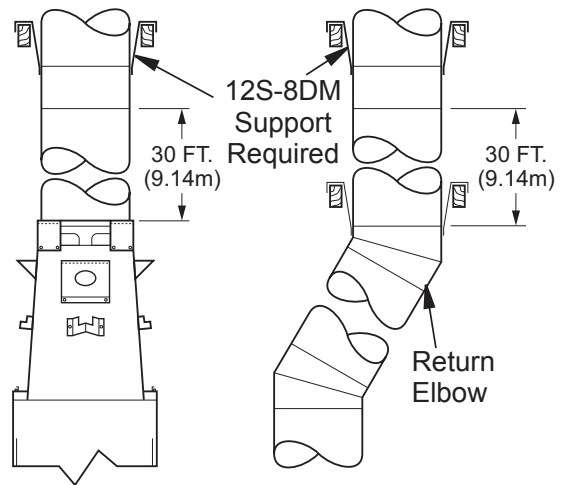
Figure 15 - Elbow Offset
