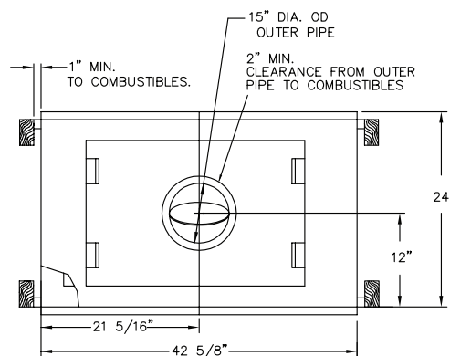
Figure 4 - Framing Firebox
