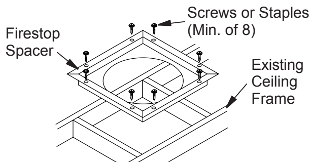
Figure 20 - Firestop Spacer with Attic Space Above Ceiling
