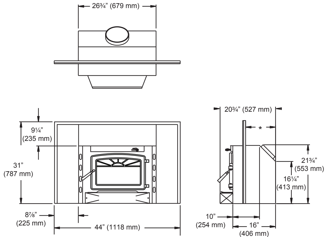
Figure 1 WR2500X02 Dimensions
