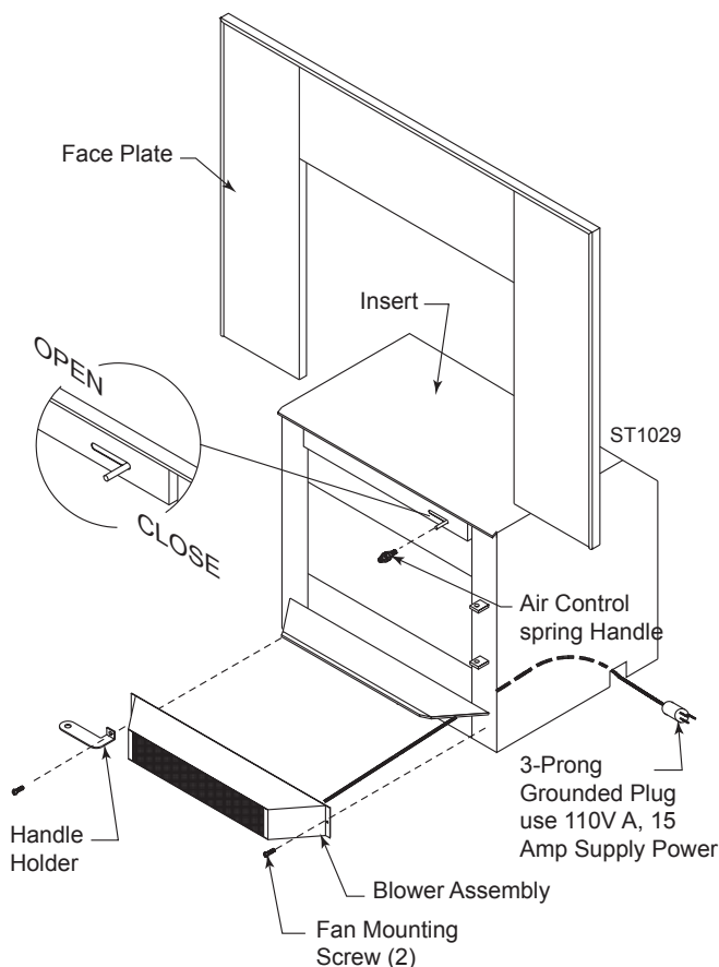
Figure 10 Blower Installation
