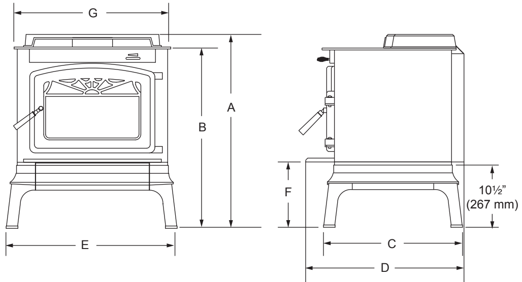
Figure 1 Stove Dimensions
