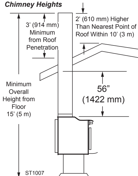
Figure 3 Chimney Heights
