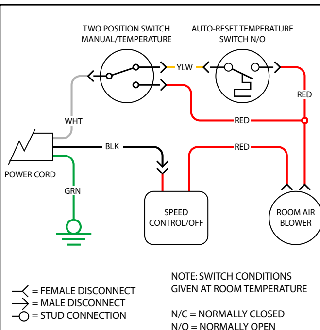
Figure 12 - Blower Wiring Schematic
