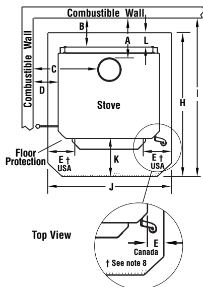
Parallel Installation
