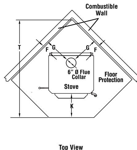
Corner Installation
