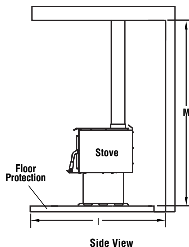
Parallel Installation
