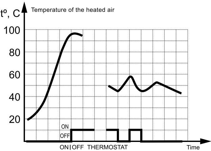
CHARACTERISTIC OF THE THERMOSTAT
