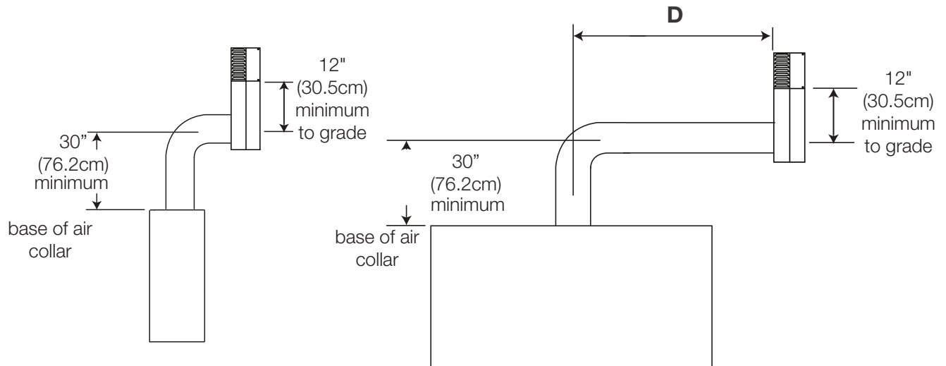
SINGLE-SIDED
