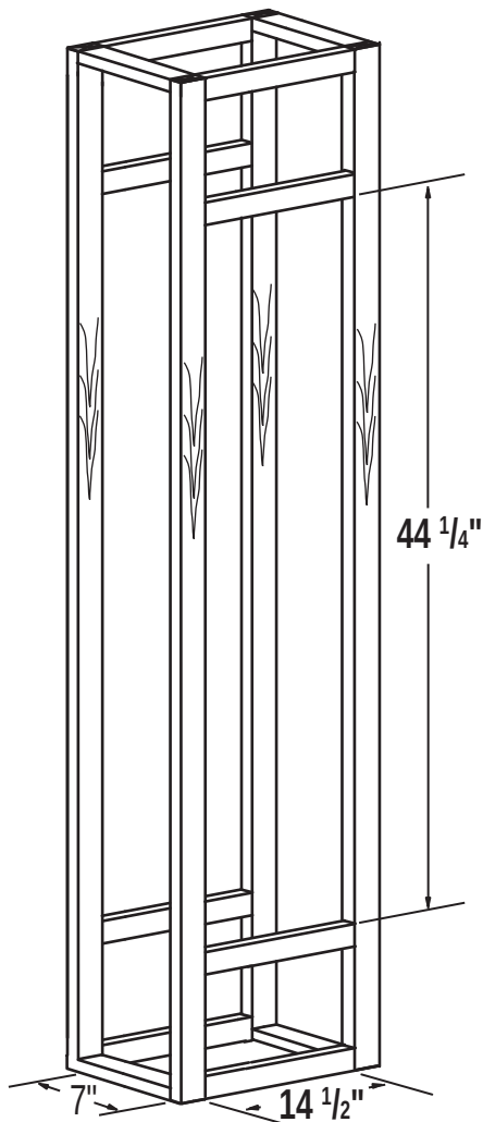
FRAMING OPENING DIMENSIONS
