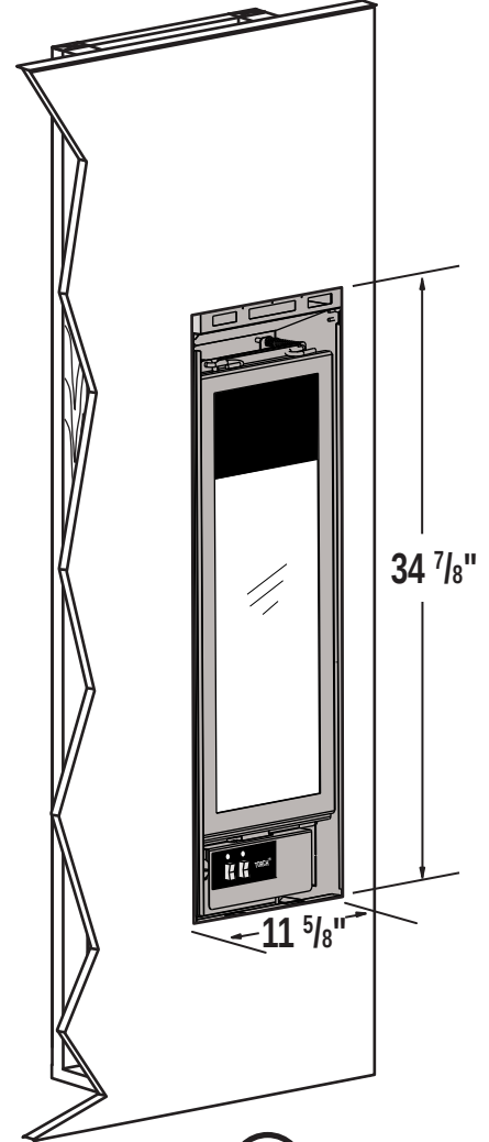
FINISHING OPENING DIMENSIONS
