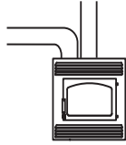
GRAVITY VENT OPTION (1 DUCT)
