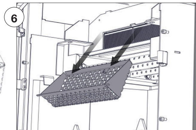
Remove the perforated catalyst shield.
