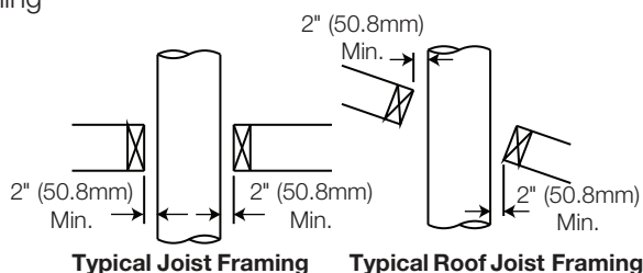
Typical Joist Framing
