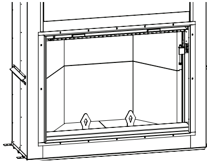
E. Install the remaining top firebricks, securing under the retaining brackets. Install the andirons into the bottom firebricks.
