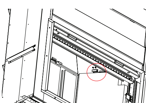
D. Tilt the top right firebrick and secure under the retaining bracket.
