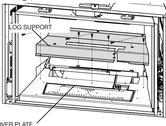
COVER PLATE
