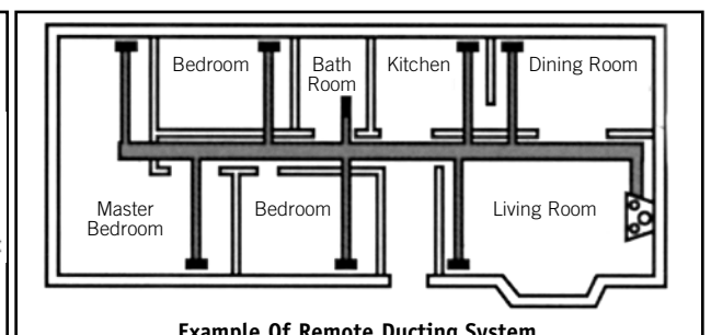
Example Of Remote Ducting System
