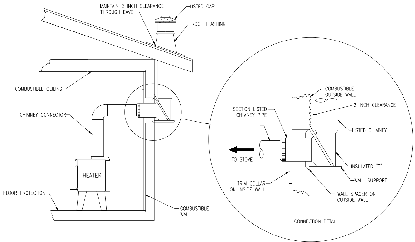
FIGURE 2.2.1 (A) Typical installation through the wall
