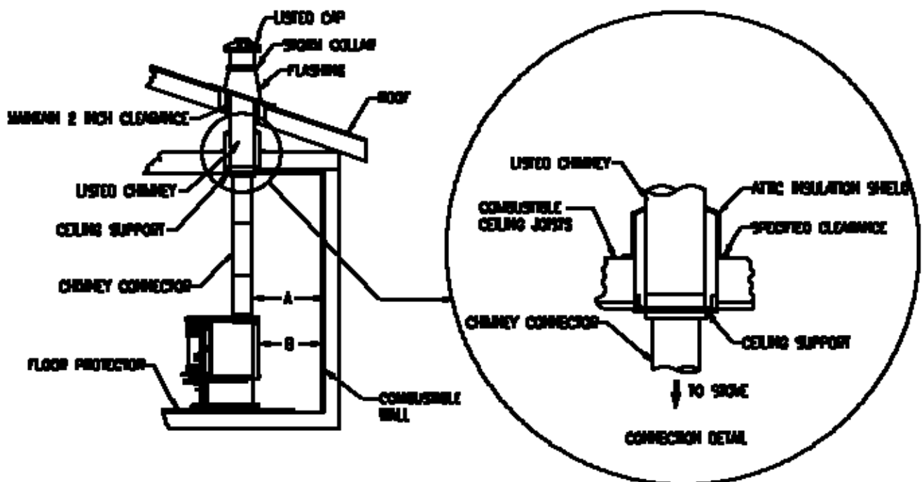
FIGURE 4 Connection to a Factory Built Chimney (Interior Shown)
