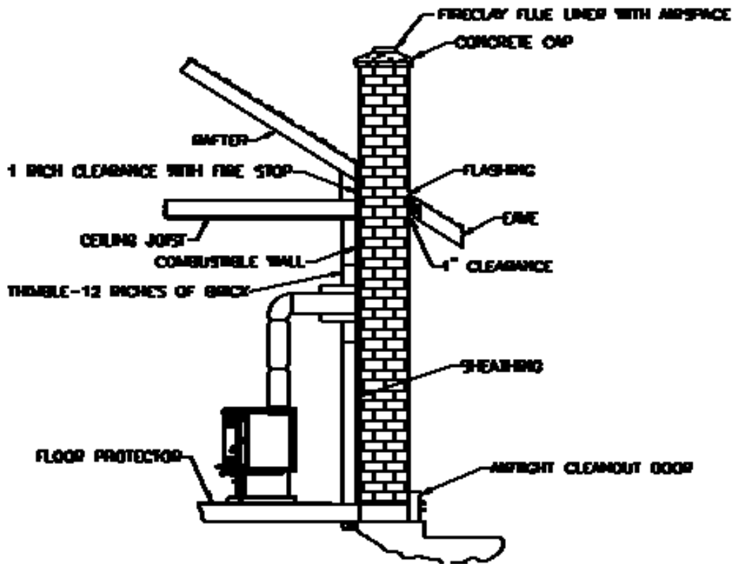
FIGURE 3.1 Connection to a Masonry Chimney (Exterior Shown)
