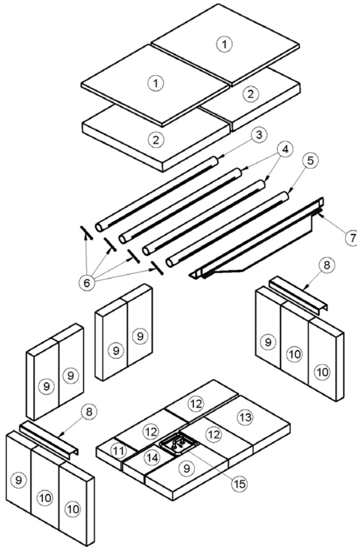
FIGURE 10 – Firebrick layout
