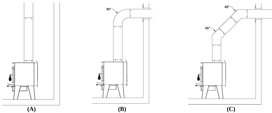
FIGURE 2.2 The use of elbows
