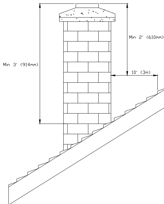
FIGURE 3 – Chimney height
