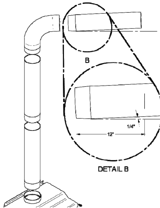
FIGURE 2.1 (B) Minimum Slope
