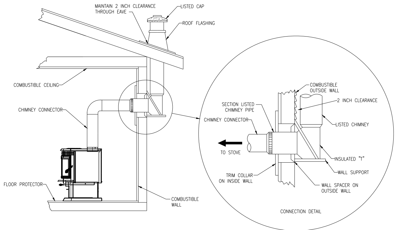
FIGURE 5 Connection to a Factory Built Chimney (Exterior Shown)
